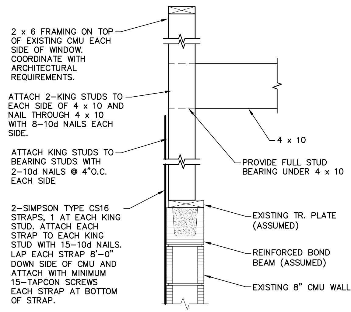
SECTION 1A 1"=1'-0" S4 | S10A
